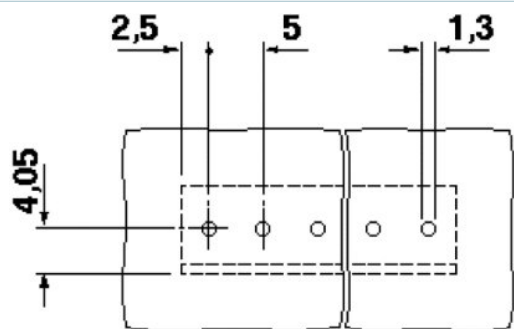
Drilling diagram
